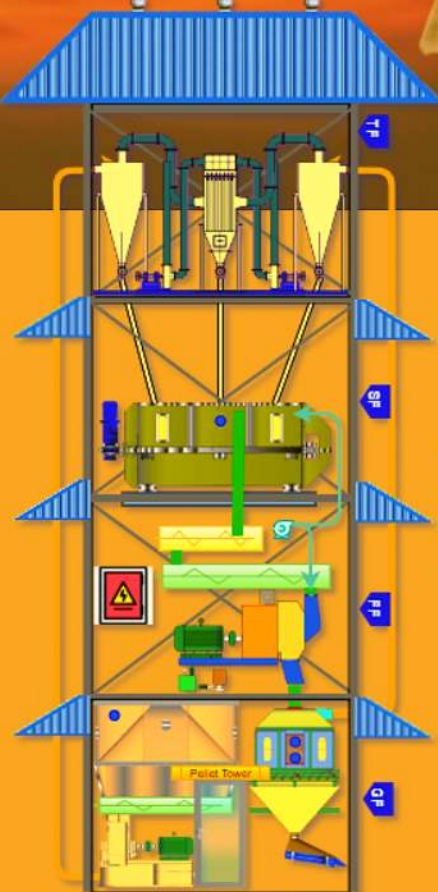
PELLET TOWER
